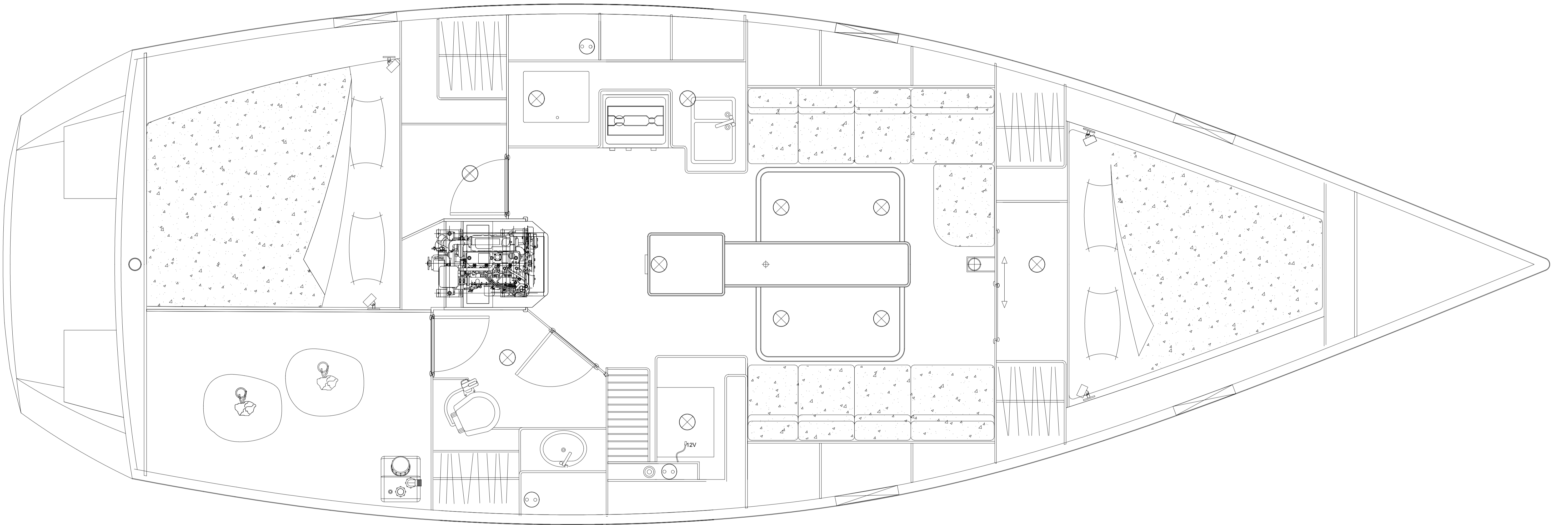
VERSION STANDARD
